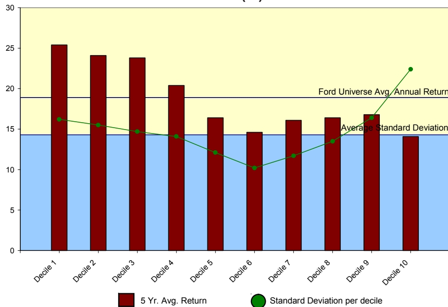
EMO Decile Returns (%) 12/02 to 12/07
